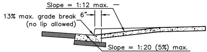
Section View
