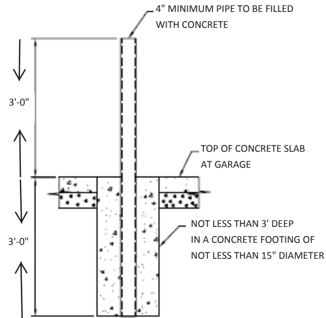
BOLLARD POST TYPICAL
